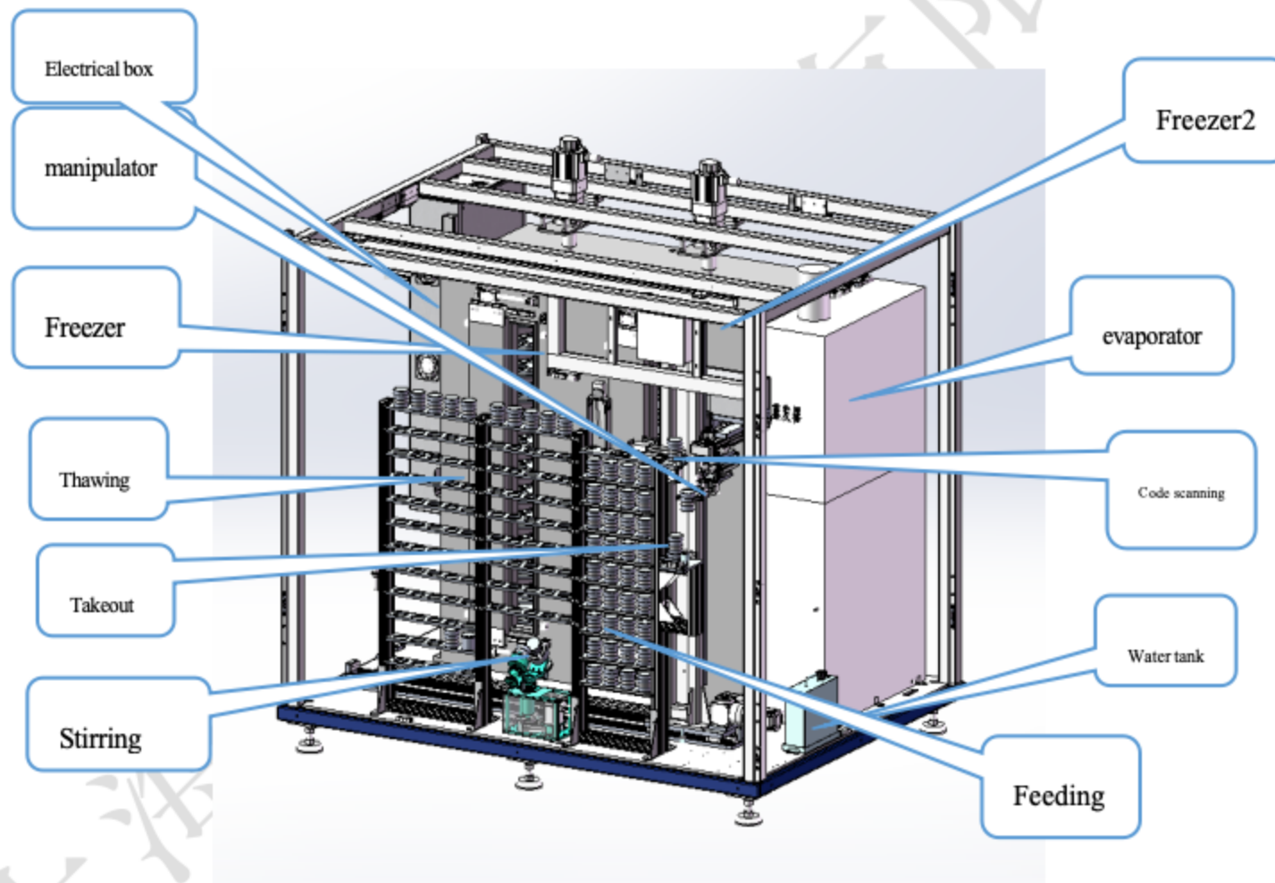
Fig.1 Schematic diagram of the shape of the solder paste cabinet
