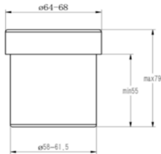
Fig.3 Solder paste bottle size
