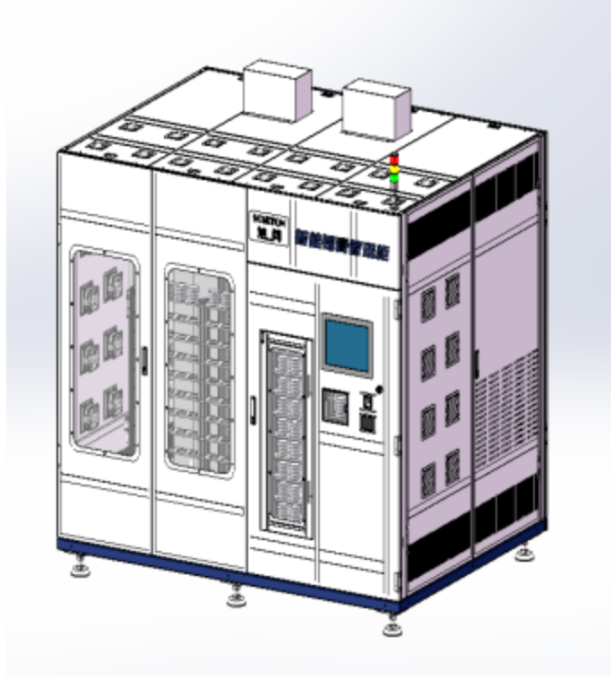
Figure 2 Appearance of the solder paste cabinet
